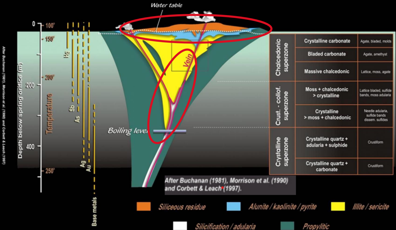
LOW SULFIDATION EPITHERMAL MODEL
