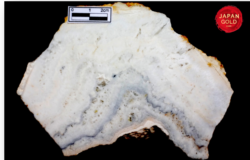
Ginguro banded quartz vein. Collected from the Kitano-o Prospect located in the Ikutahara Project . 60.8 g/t Au and 89.6 g/t Ag.
