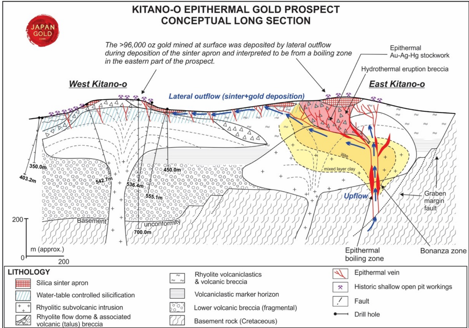
Figure modified from Sillitoe, 1992. Appraisal of Epithermal Gold Prospects and Exploration Approach in the Northern Hokkaido Area, Japan This model is largely based on Dr Sillitoe's observations at the Kitano-o Mine area on Japan Gold's Ikutahara Project
